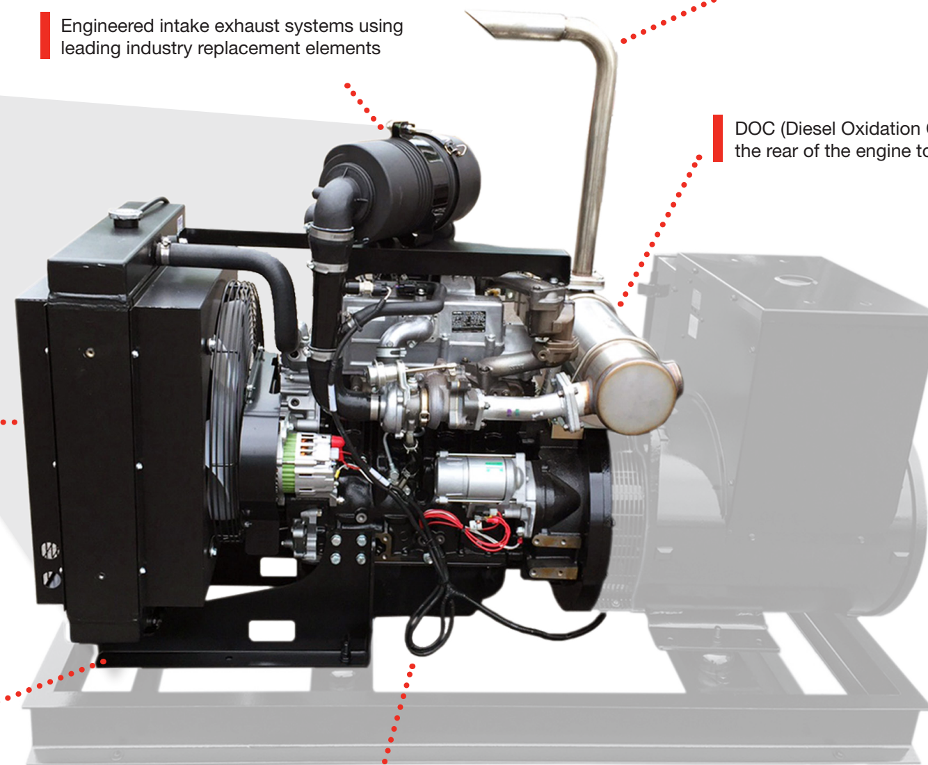
4LE2 Power Unit with Generator Attachment
